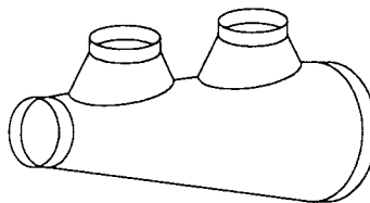
TRANSITION WITH CONICAL TAPS
