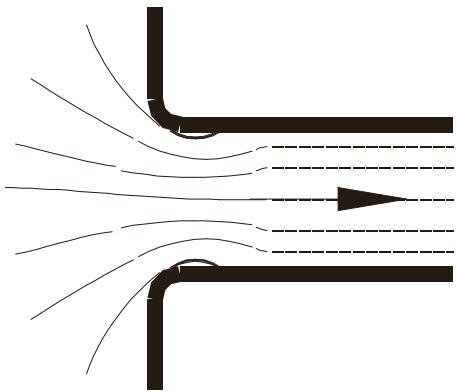
SLIGHTLY ROUNDED K_e = 0.23
