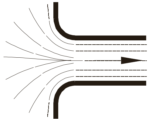
BELL MOUTH K_e = 0.04
