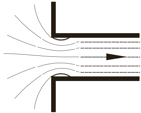
SQUARE ENTRANCE K_e = 0.50
