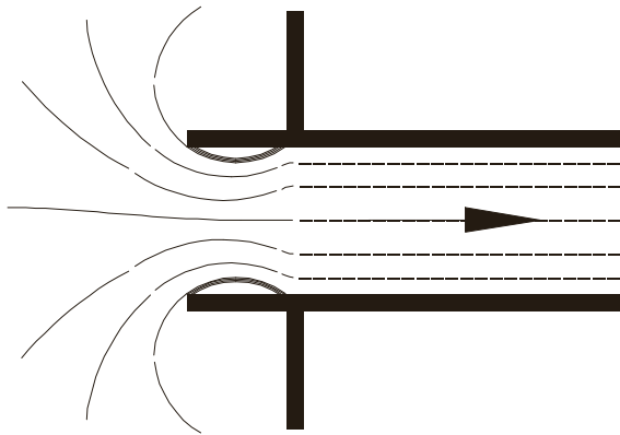
INWARD PROJECTING K_e = 0.78
