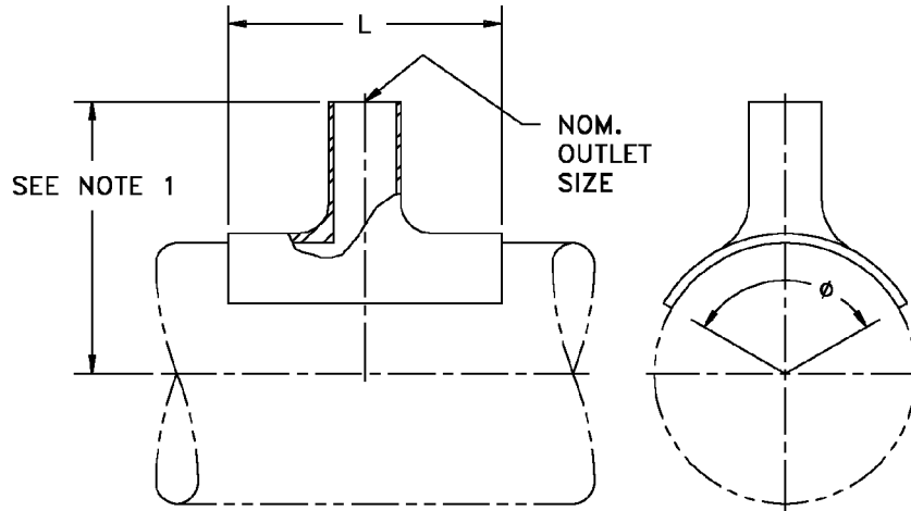
FIG. #62 - Reducing Saddle with Plain End Pipe Stub Outlet
