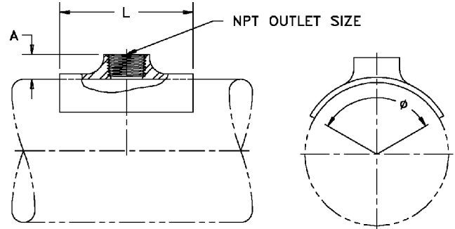
FIG. #60 - Reducing Saddle with Fiberglass NPT Threaded Outlet
