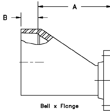
FIG. #56 - Eccentric Tapered Body Reducer, Combination Coupled
