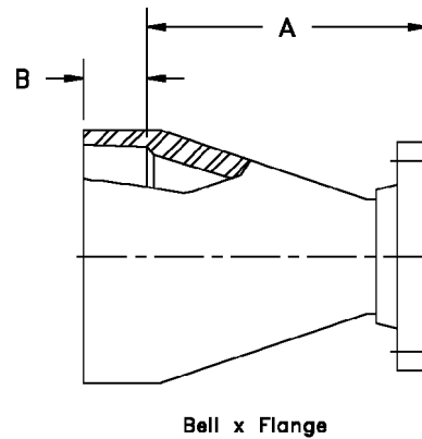
FIG. #55 - Concentric Tapered Body Reducer, Combination Coupled
