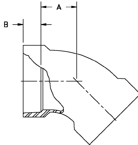
FIG. #30-25 - 45 Degree Elbow, Bell End (25 psi or Duct Rated)
