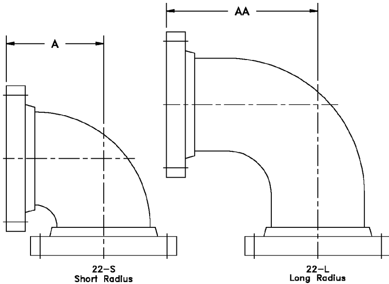
FIG. #22-S/22-L - 90 Degree Elbow, Short or Long Radius, ANSI 150 lb. Flanged
