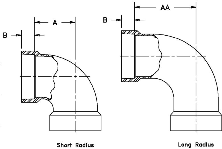
FIG. #20-25 - 90 Degree Elbow, Short or Long Radius, Bell End (25 psi or Duct Rated)
