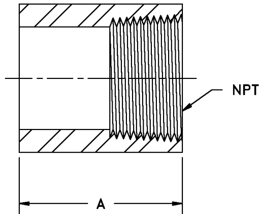
FIG. #2-EL/2 - Threaded Extra Long Half Coupling, Female NPT
