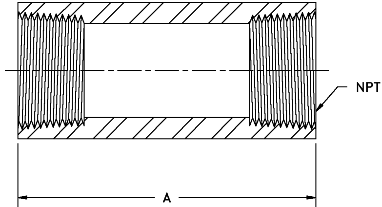
FIG. #2-EL - Threaded Extra Long Coupling, Female NPT
