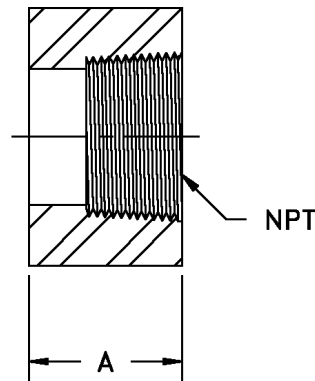
FIG. #10 - Threaded Reducing Bushing, Spigot x Female NPT
